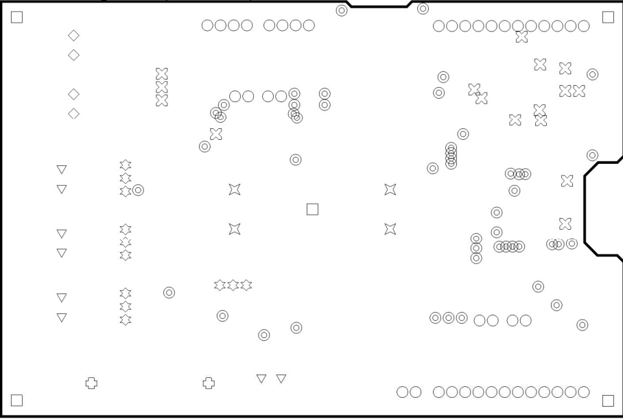
Drill Drawing View (Scale 1:1)
